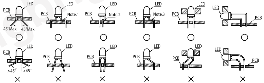
" ○ " Correct mounting method " X " Incorrect mounting method
